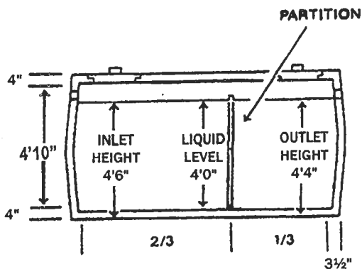
CROSS SECTION
