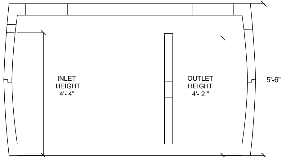
CROSS SECTION
