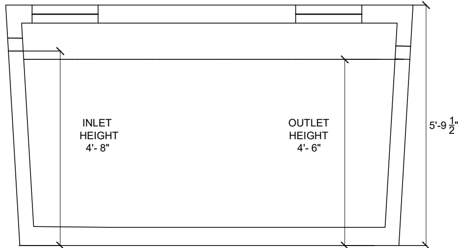
CROSS SECTION
