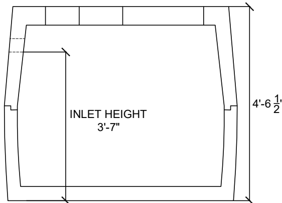
CROSS SECTION
