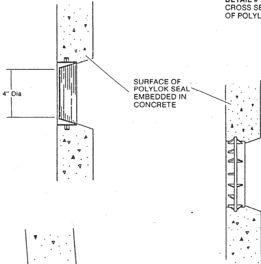
DETAIL # W8•002 CROSS SECTION OF SEPTIC TANK JOINT AND RUB'R NEK SEAL:
