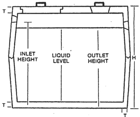
CROSS SECTION
