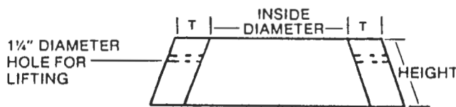
24" (600 mm) - 32" (800 mm) Inside Diameter TAPERED CONE
